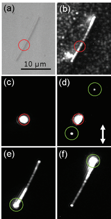
Figure 3. (a) White light transmission image of an Ag NW. (b) QD emission image with wide-field excitation. (c) The image with 710 nm laser focused on the position marked with a red circle as in (a) and (b). (d) Emission image acquired using an 800/30 nm band-pass filter and with an excitation wavelength of 710 nm. The laser is focused on the same position as in (c) but with a higher power level of 200 \mu W. The exposure time is 5 s. The white arrow indicates the polarization of the laser. (e) and (f) QD emission images obtained by focusing a 710 nm wavelength laser on the wire ends marked with green circles.
